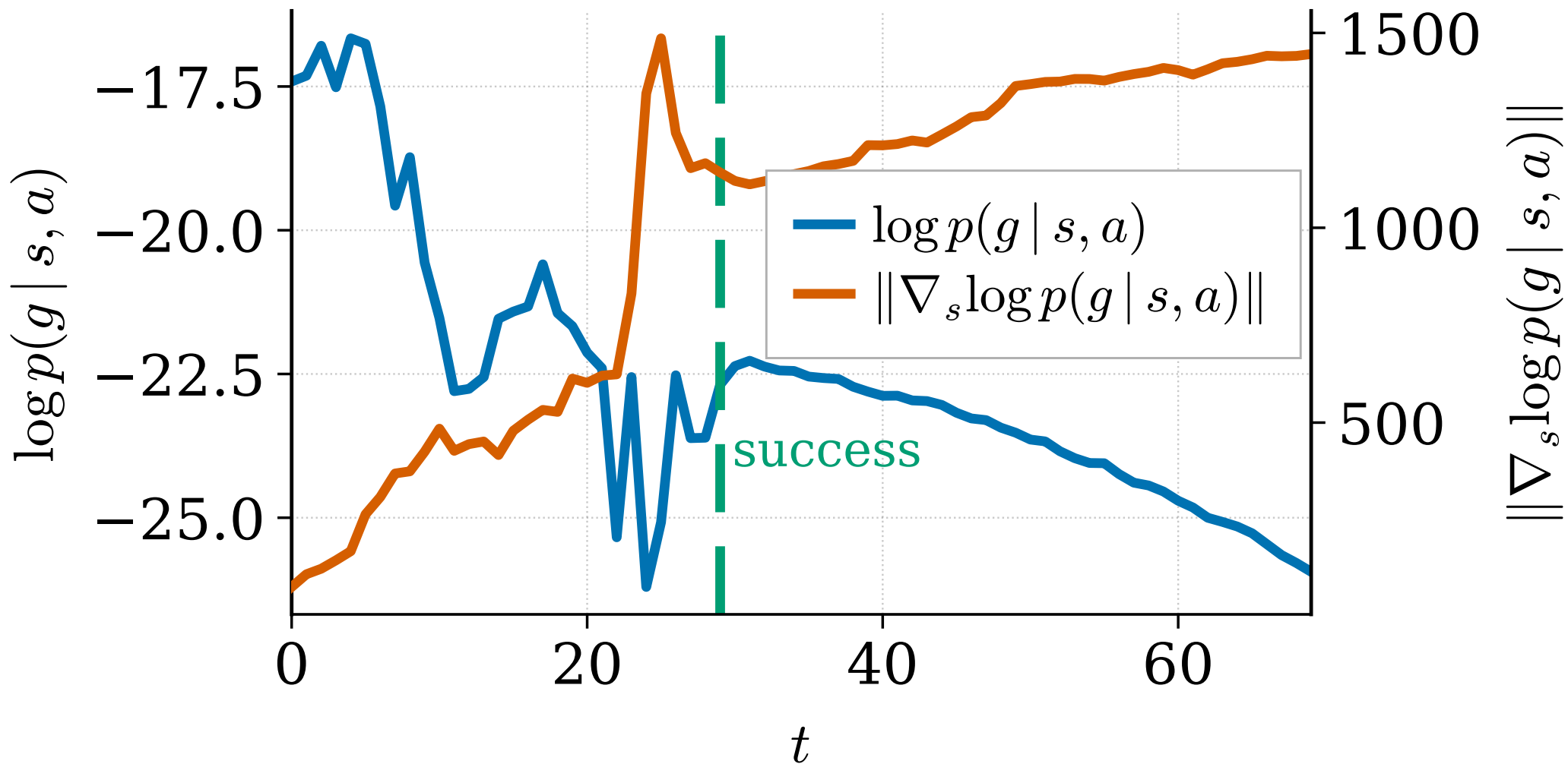
NF log likelihood after success
